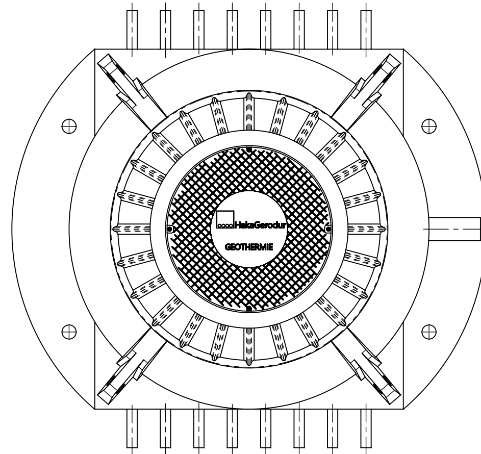
Kunststoffdeckel A15 verschraubt Couvercle en plastique A15 boulonné Coperchio in plastica A15 imbullonato Plastic cover A15 bolted
