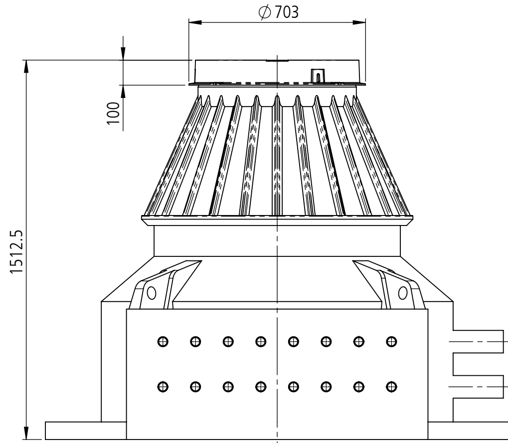
Vollguss Abdeckung B125 verschraubt Couvercle en fonte B125 boulonné Coperchio in ghisa B125 imbullonato Cast iron cover B125 bolted
