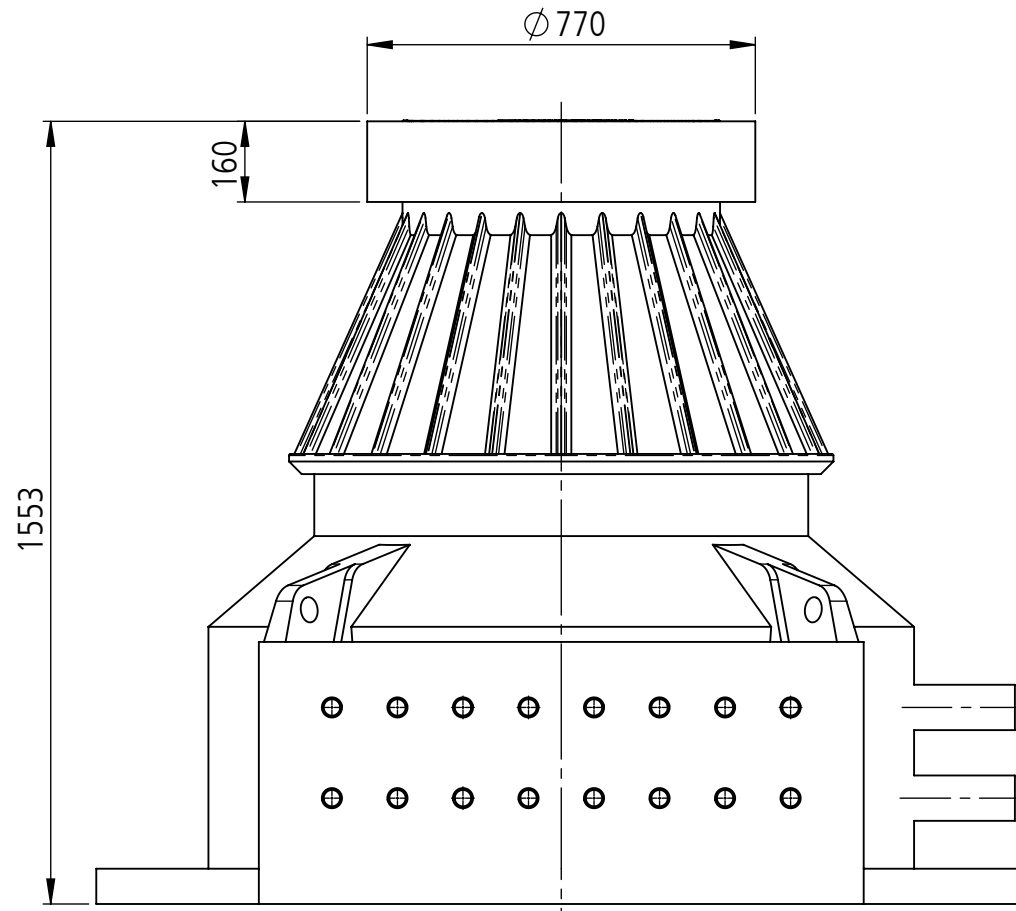
Kunststoffdeckel A15 verschraubt Couvercle en plastique A15 boulonné Coperchio in plastica A15 imbullonato Plastic cover A15 bolted
