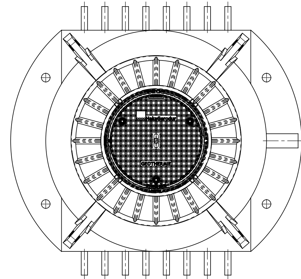
Vollguss Abdeckung B125 verschraubt Couvercle en fonte B125 boulonné Coperchio in ghisa B125 imbullonato Cast iron cover B125 bolted
